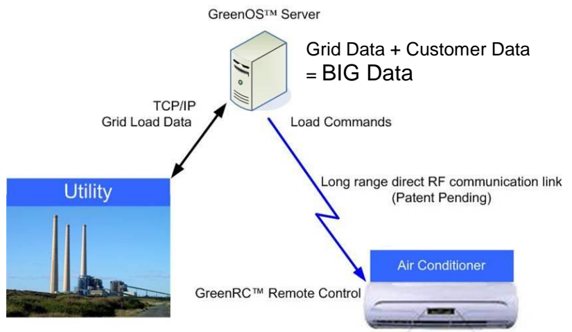
GreenRC System architecture
